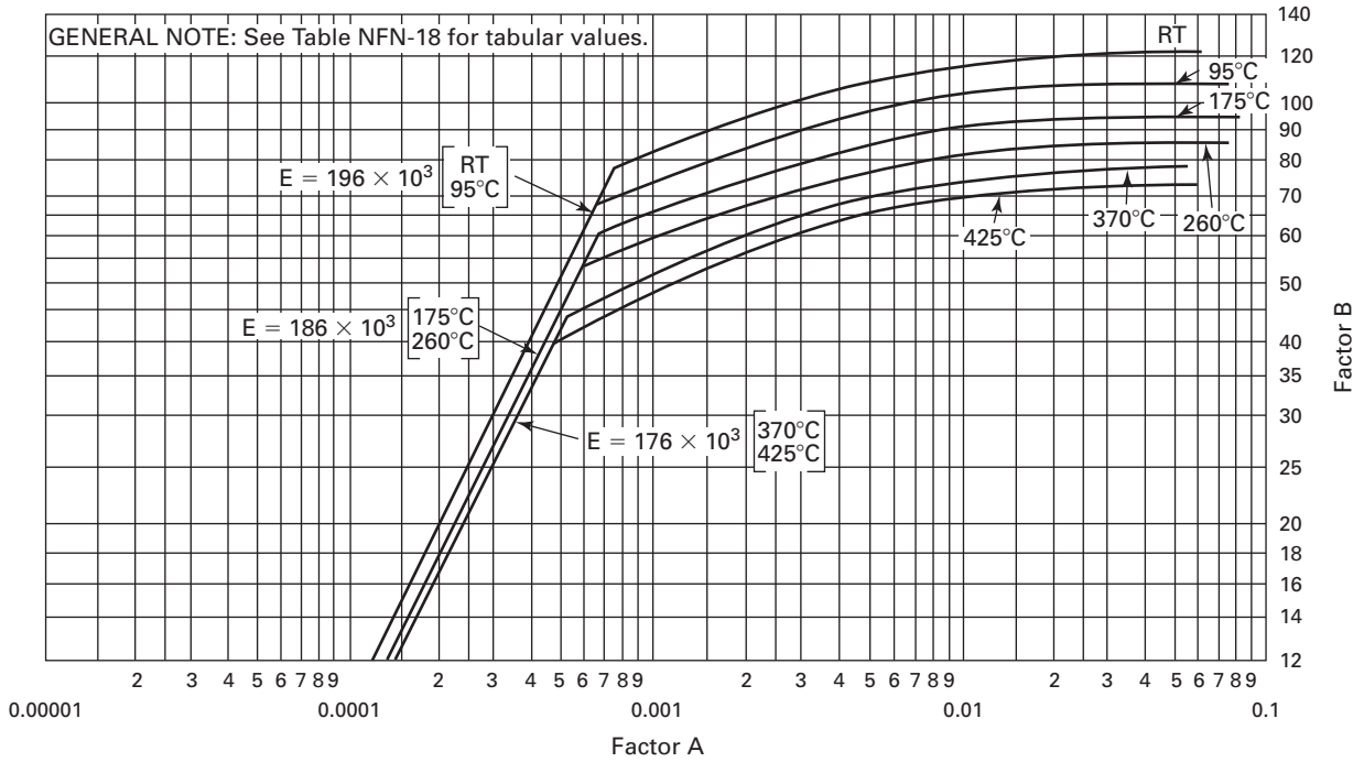
Figure NFN-18 Chart for Determining Shell Thickness of Components Under External Pressure Developed for Nickel–Molybdenum–Chromium–Iron–Copper Alloy N06985 Having a Minimum Yield Strength of 240 MPa
