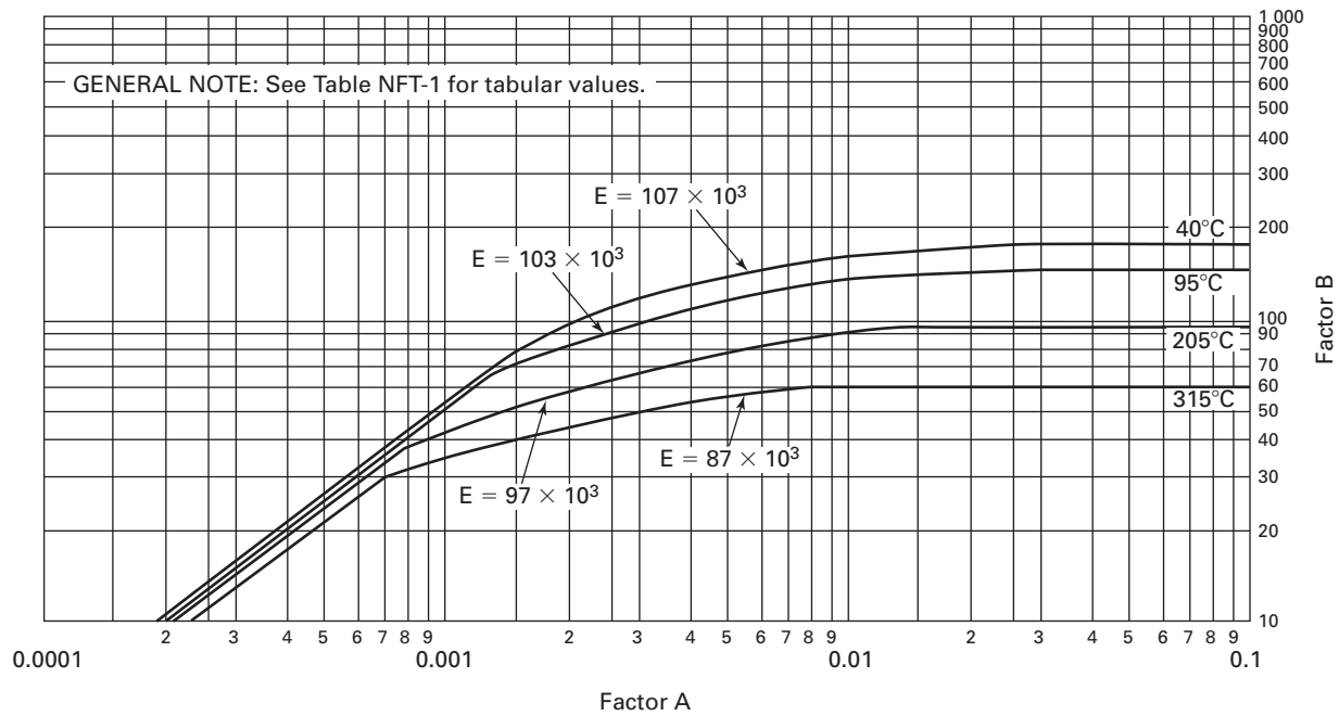
Figure NFT-1 Chart for Determining Shell Thickness of Components Under External Pressure Developed for Unalloyed Titanium Grade 3 (UNS R50550)
